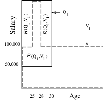
Figure 1: Semantic Spaces
