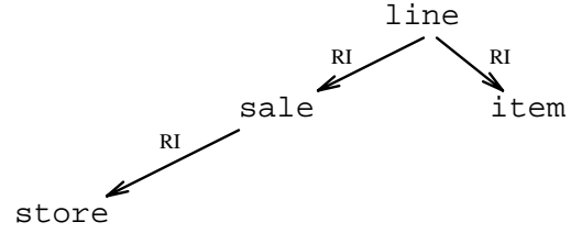
Figure 2: Join Graph G(\text{cal\_toy\_sales})
