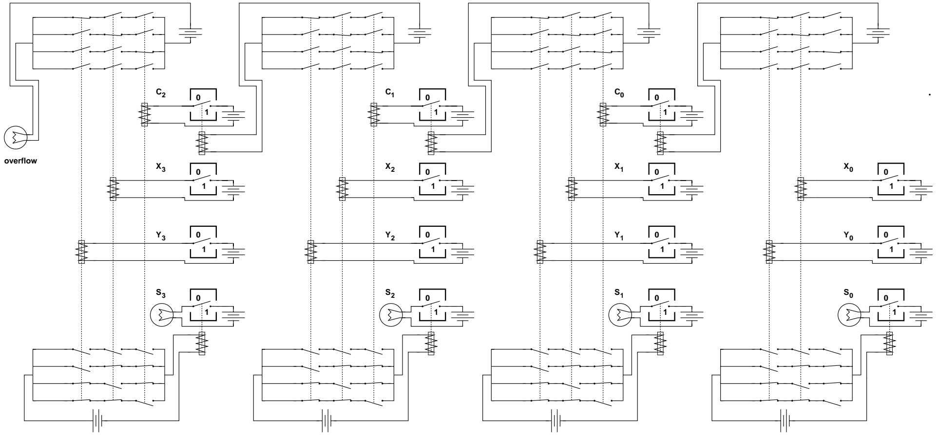
Four bit adder without decoder and control
