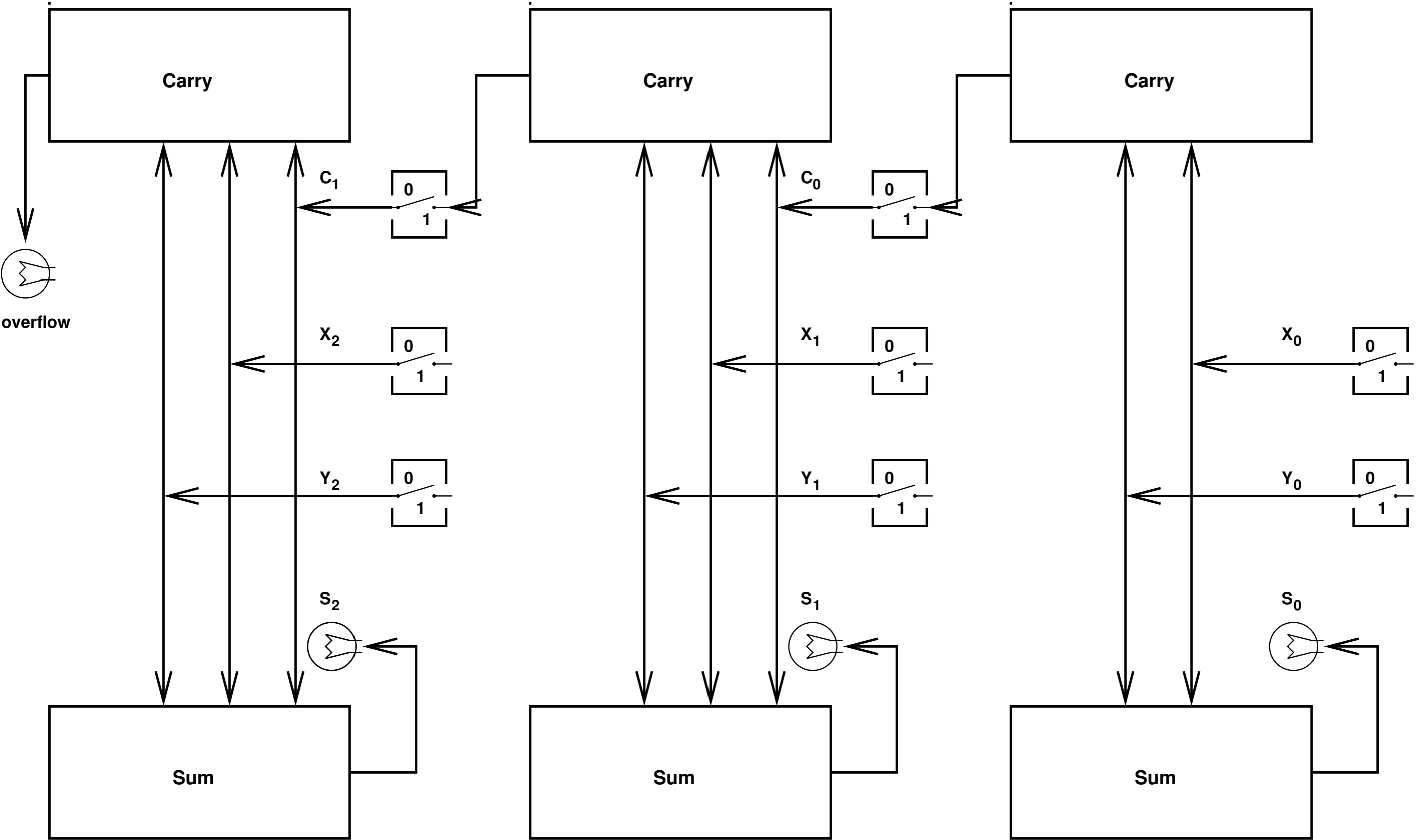
Block Diagram for a Three Bit Adder
