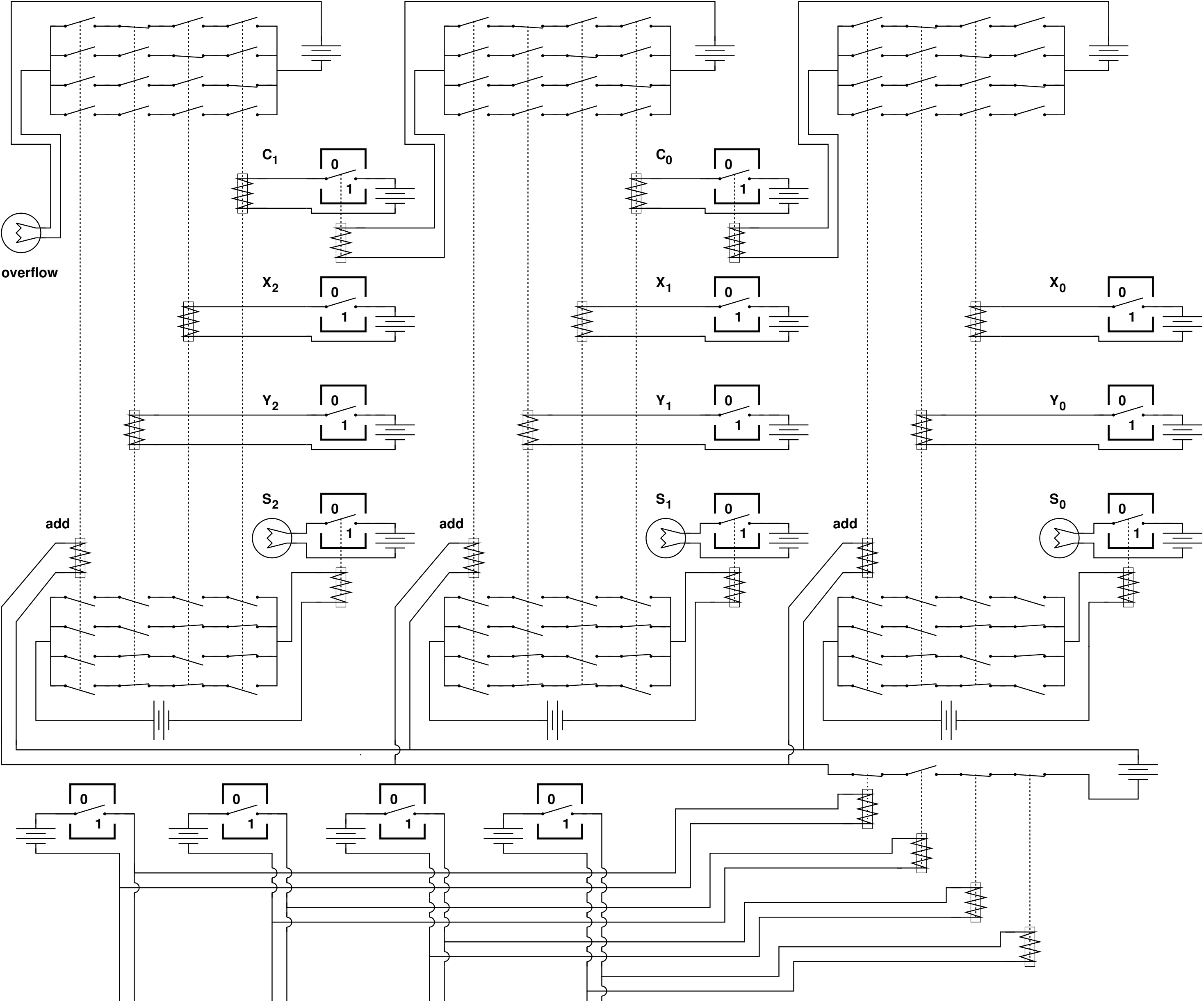
Three Bit Binary Adder
