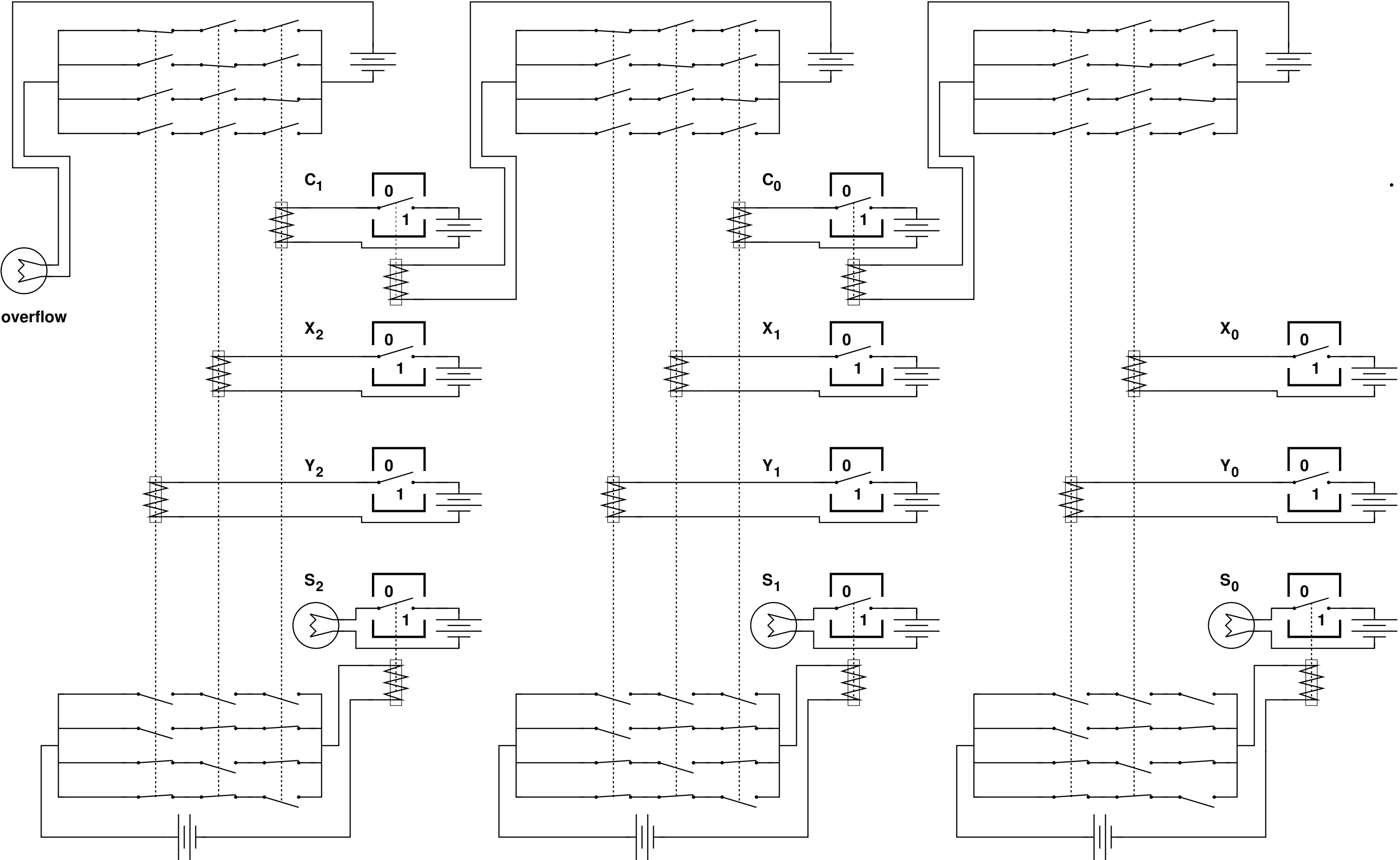
Three bit adder without decoder and control
