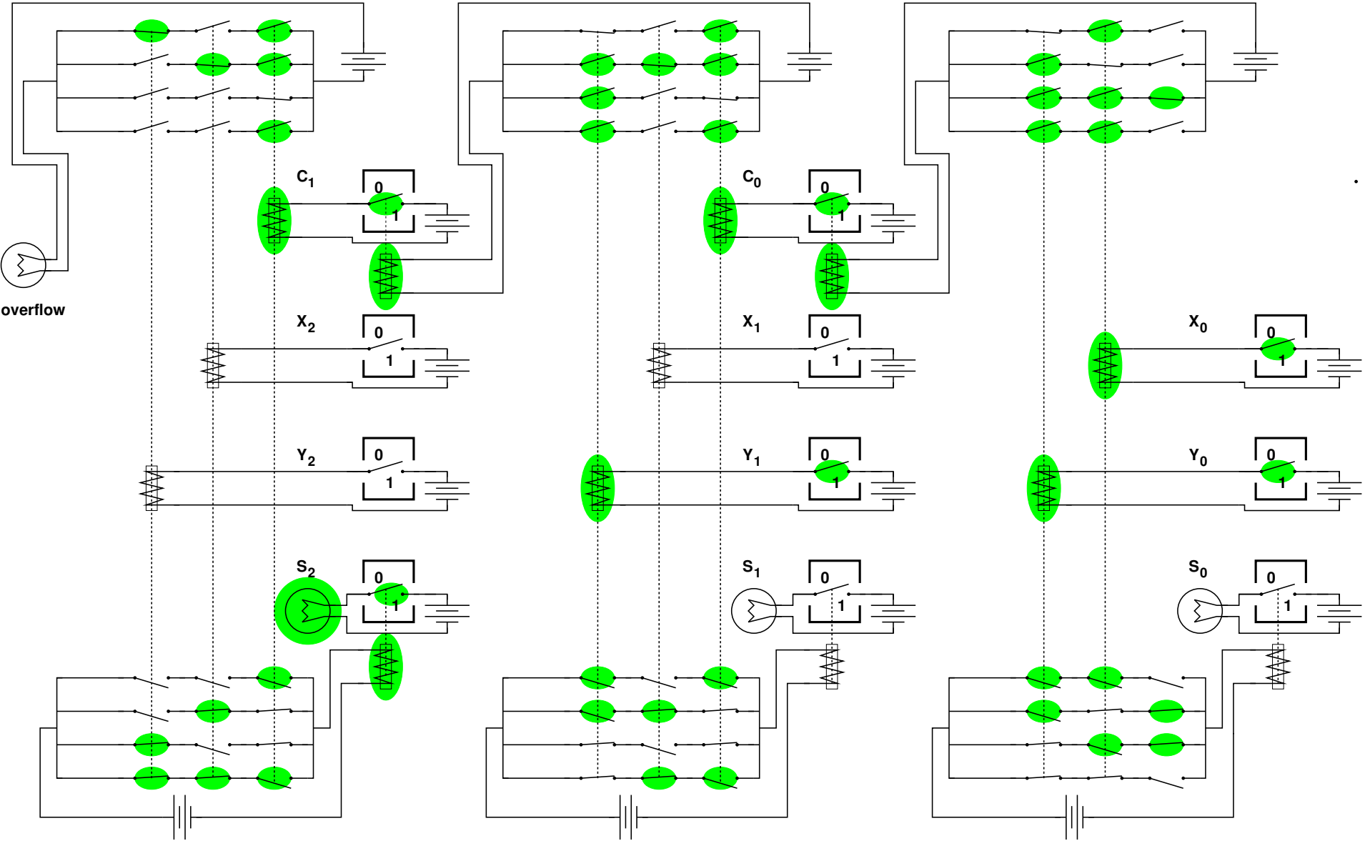
Three bit adder without decoder and control
