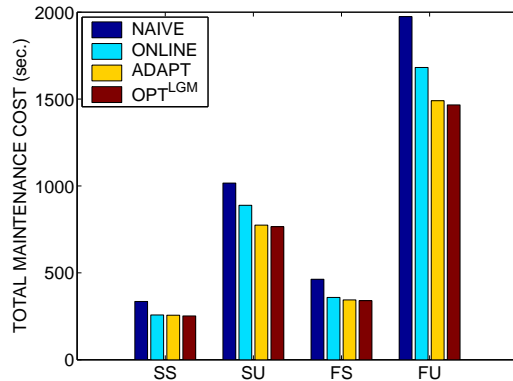
Figure 7. Non-uniform arrivals.
