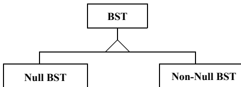
Figure 2 BST’s modeled in an inheritance hierarchy
