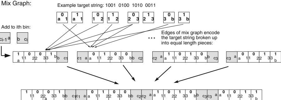
Fig. 7 This tileset and mix graph depict a tile system with 2w tiles and w bins that will assemble an arbitrarily specified length w^2 binary string
