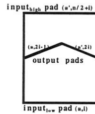
Figure 7c: A square tile for perfect shuffle, with middle segment used for output.
