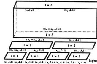
Figure 5b: Stage t=3 of 3D parallel prefix assembly: computation of b_4 .
