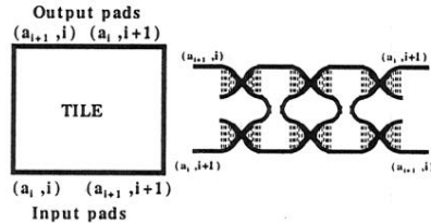
Figure 7a: A square tile for pair-wise exchange and a DNA DX nano-structure for the tile.
