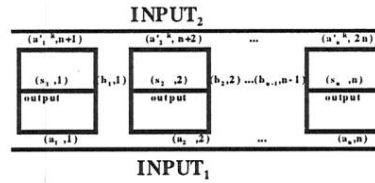
Figure 3d: 2D assembly for bit-serial addition.
