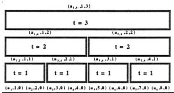
Figure 4e: Final step t = 3 of assembly for parallel monoid sum computes b_8 = a_{1,8} = a_1 \cdot a_2 \cdot \dots \cdot a_8 .
