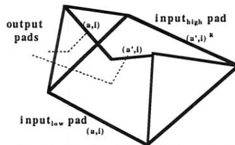
Figure 7e: Alternative 3D polyhedral tile for perfect shuffle.
