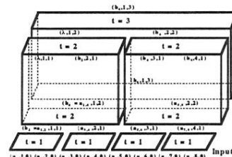
Figure 5c: Stage t=2 of 3D parallel prefix assembly: computation of b_2, b_4, and b_8 .
