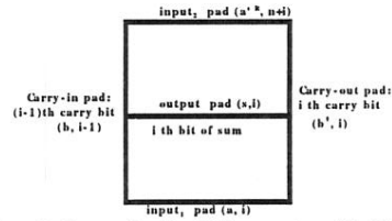
Figure 3c: Square tile with middle segment, used for bit-serial addition.
