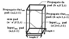
Figure 5a: A 3D polyhedron tile for parallel prefix computation.
