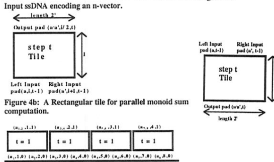
Figure 4c: Step t = 1 of step-wise assembly for parallel monoid sum computes a_{i,t+1} = a_i \cdot a_{i+1} for odd i.
