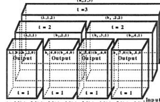
Figure 5d: Final stage t=1 of 3D parallel prefix assembly: computation of b_1, \dots, b_7 .
