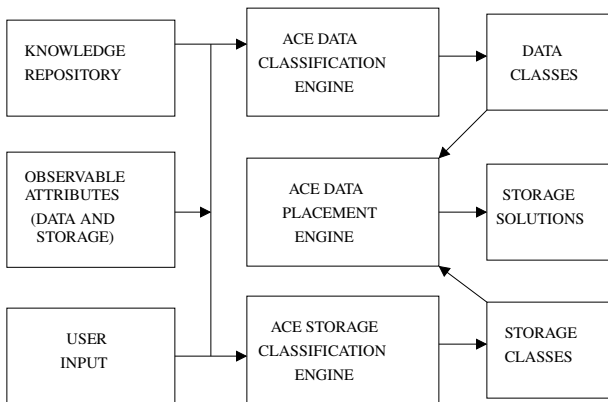
Figure 1. ACE architecture
