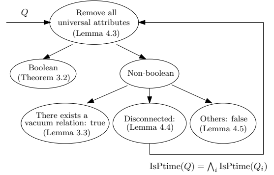
Figure 3: Procedure \text{ISPTIME}(Q) .
